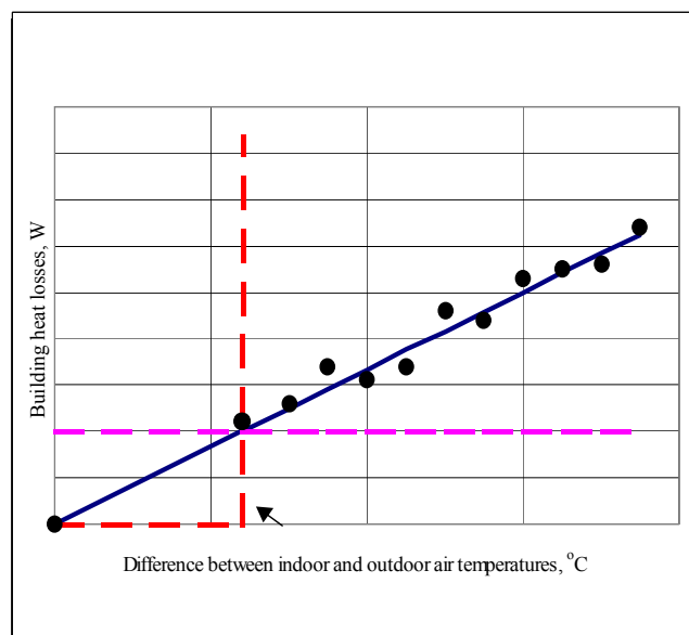
Figure 2. Functional relationship between building heat losses and temperature differences between indoor and outdoor air
